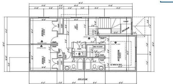
UPPER FLOOR PLAN 805 sq. ft.
