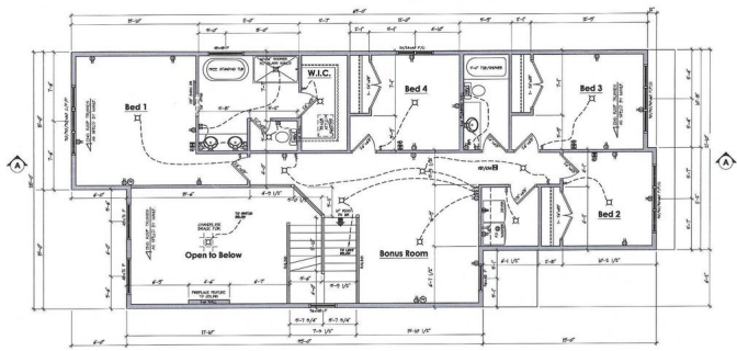
Second Floor Plan 1206 sq ft 8'7" Ceiling
